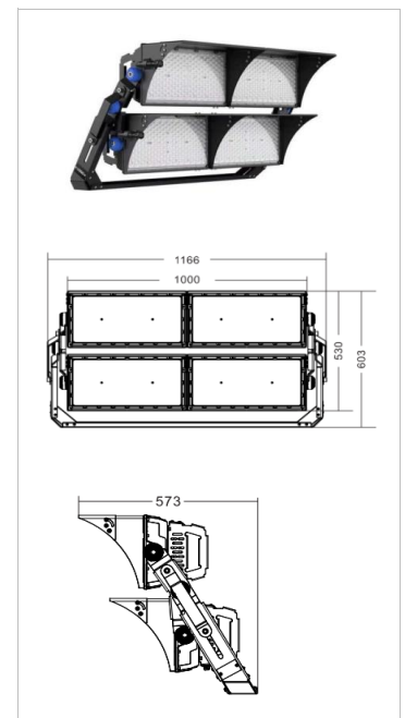
SL-01D-2000W
