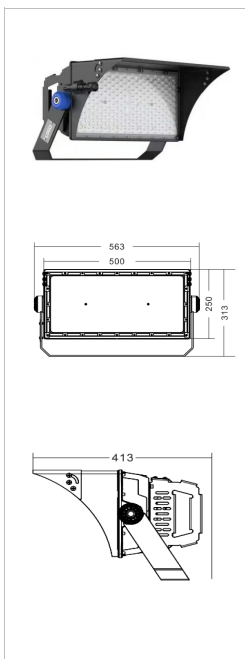
SL-01A-500W
